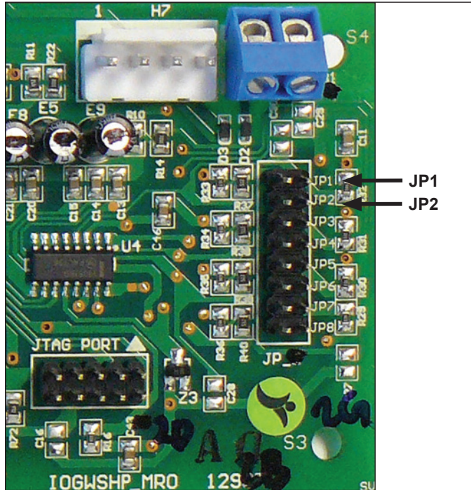
Figure 8: JP1 &amp; JP2 location on the I/O expansion module
