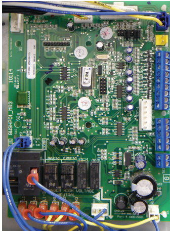
MicroTech Controller
