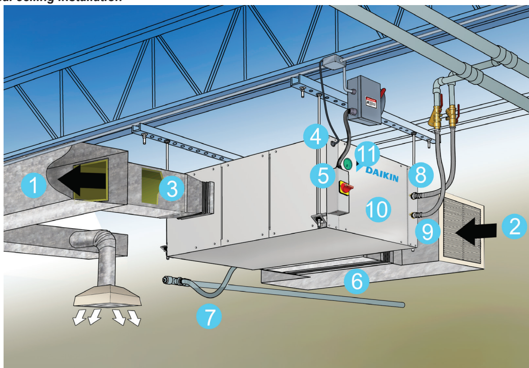
Figure 5: Typical ceiling installation
