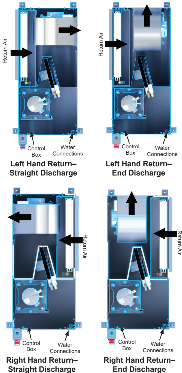
Figure 1: Four horizontal unit configurations
